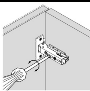
Height adjustment via mounting plate \pm 2 mm
