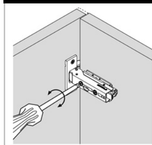
Side adjustment with limit stop \pm 2 mm
