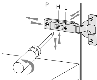
Convenient depth adjustment via worm screw \pm 3/-2 mm
