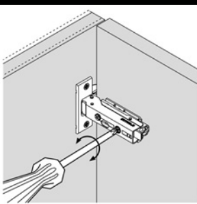
Convenient depth adjustment via worm screw \pm 3/-2 mm
